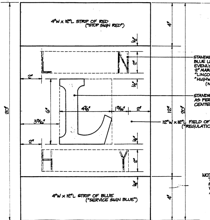
12" STANDARD SIGN (3/8 SCALE)
